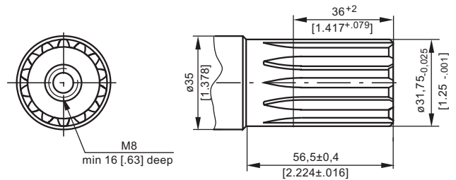
SH - \varnothing 1\frac{1}{4} " splined 14T, DP12/24 ANS B92.1-1970 Max. Torque 95 daNm [8400 lb-in]
