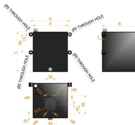
Type 5L – 7L – 10L
